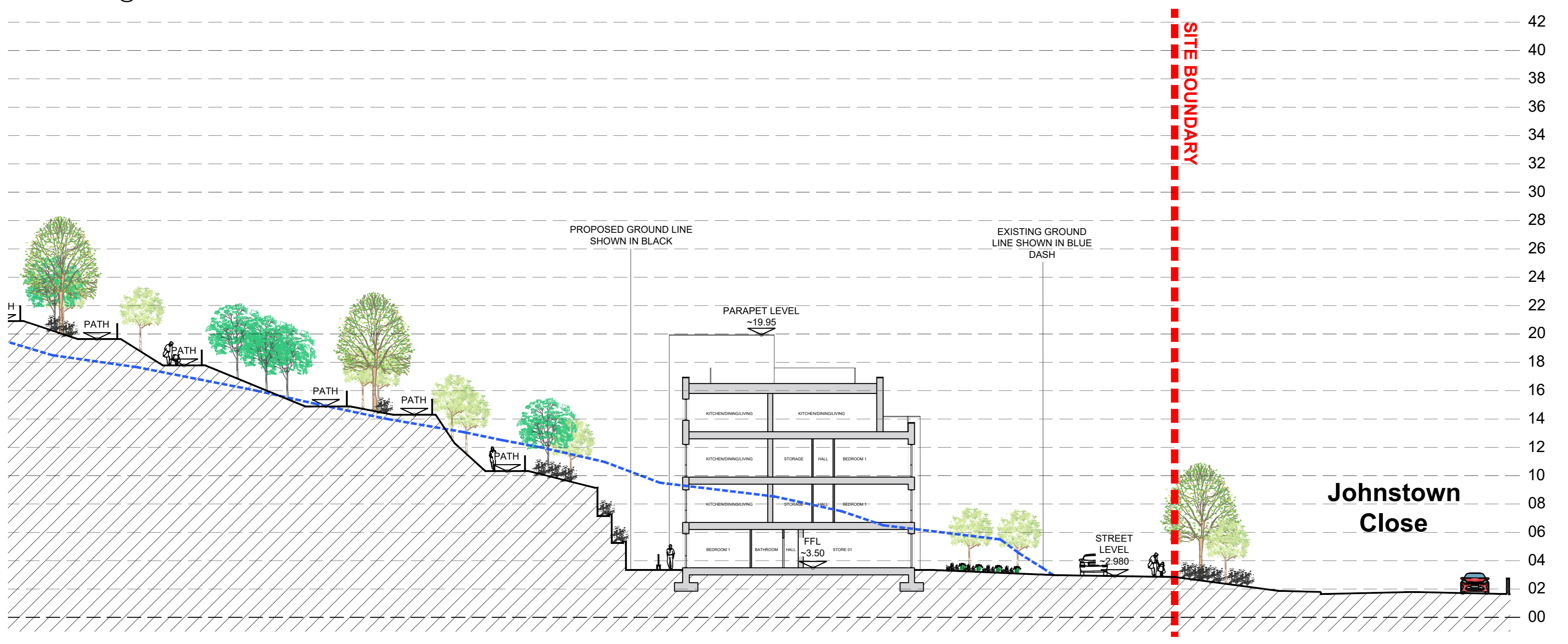
SECTION A-A (PART E) SCALE 1:200@ A0
