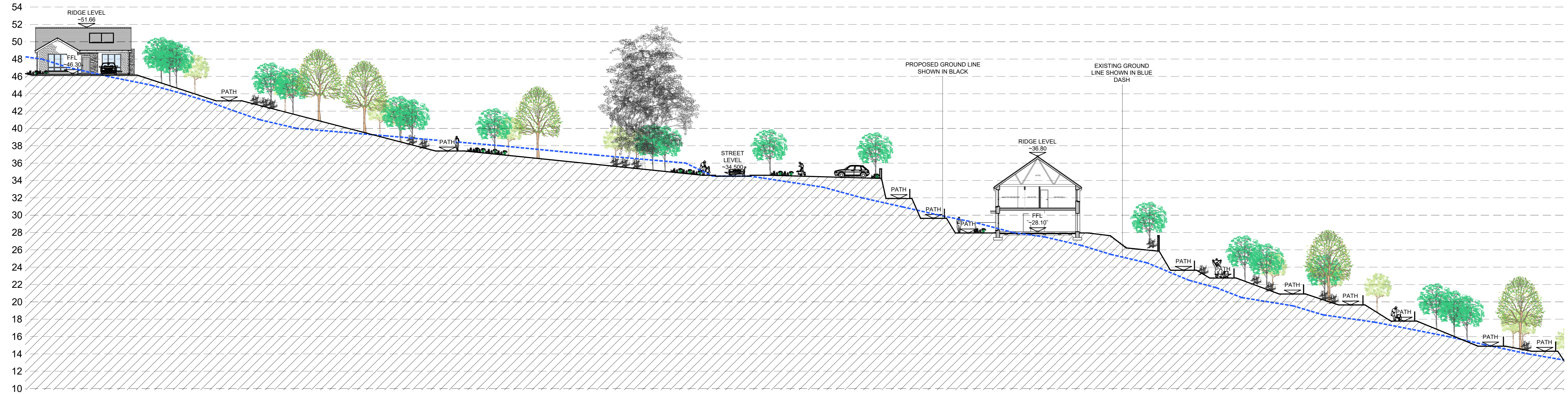
SECTION A-A (PART D) SCALE 1:200@ A0
